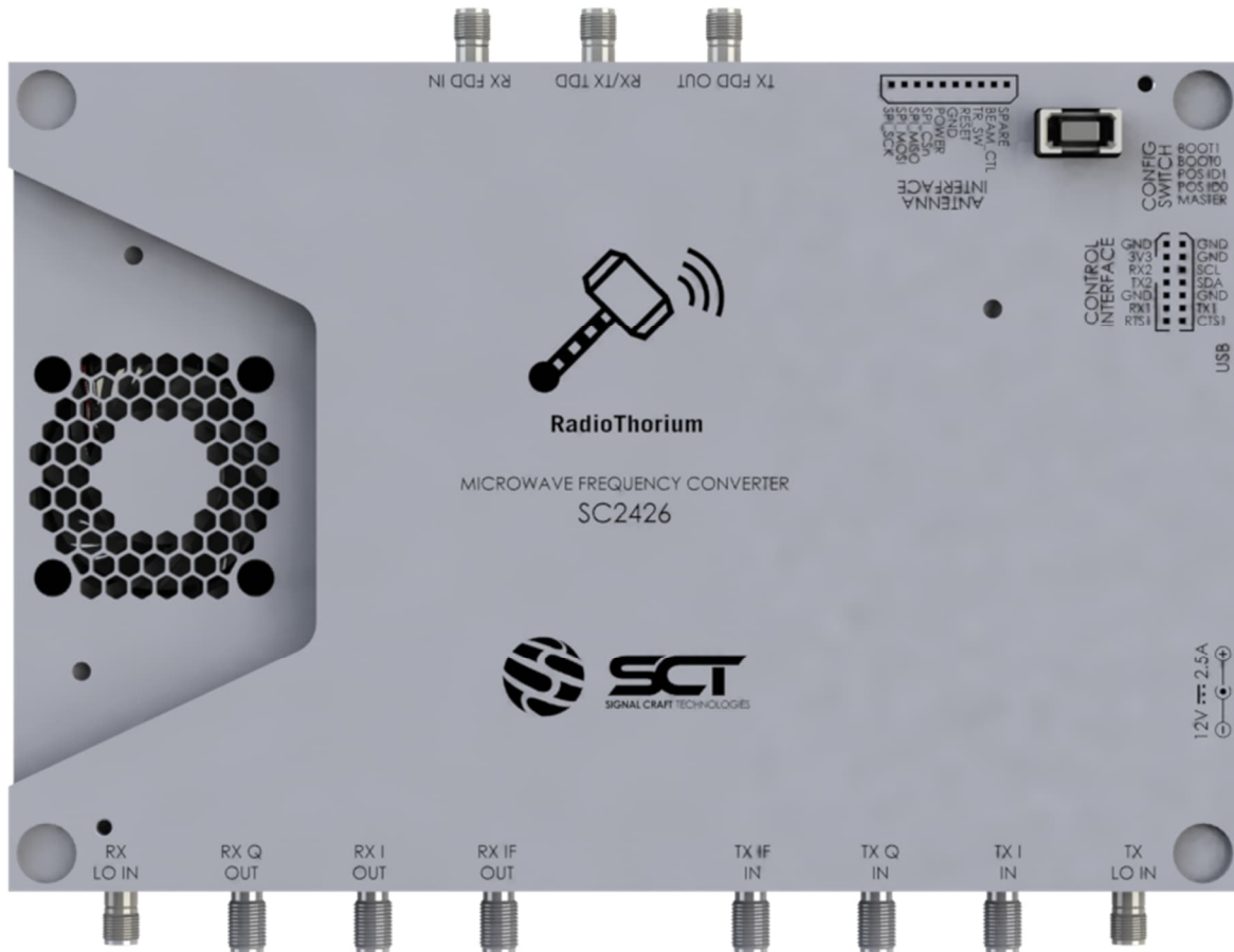
SC2426 Top View
